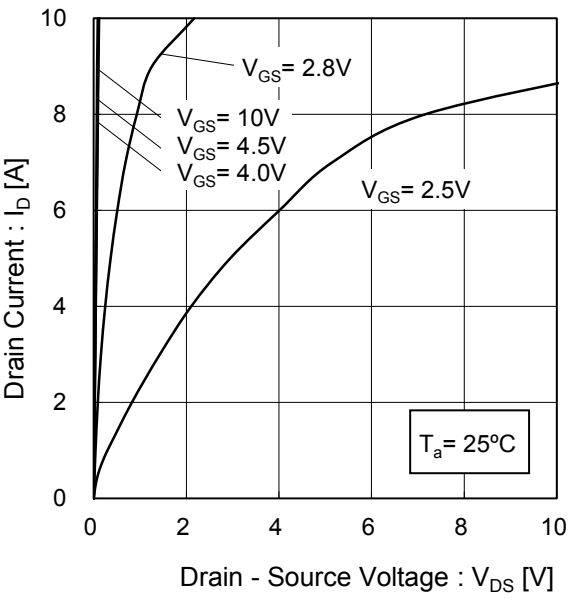
Fig.6 Typical Output Characteristics(II)
