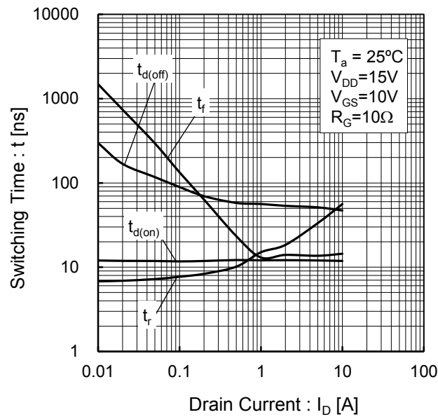
Fig.19 Switching Characteristics
