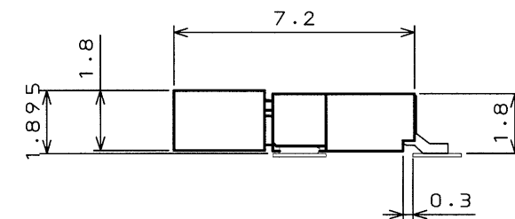
MATED CONDITION (REF.) 嵌合状態図(参考)
