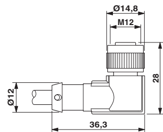
M12 x 1 socket, straight, shielded
