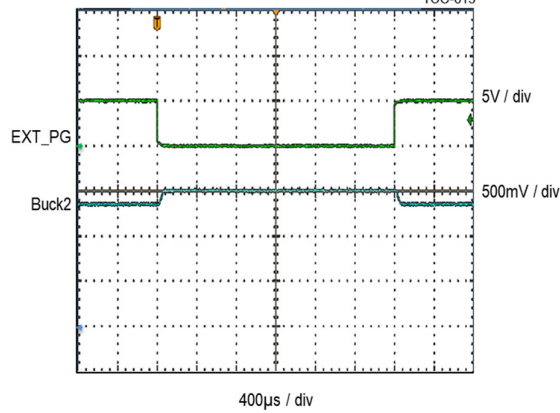
Short Circuit
