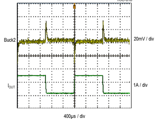
Load Transient Buck2 - Vout=1.5V 125mA to 1500mA
