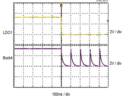
Short Circuit
