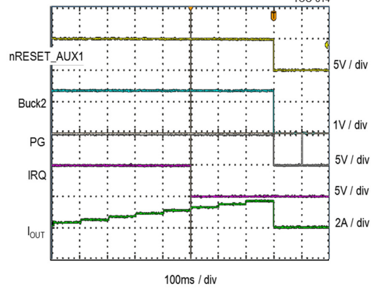
Overcurrent
