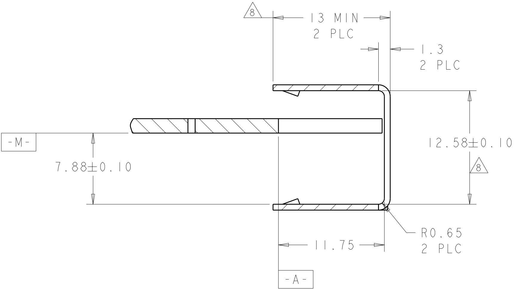
SECTION Z-Z
