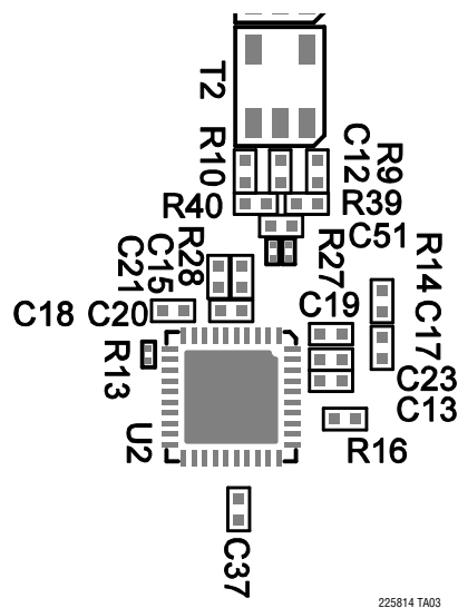
Silkscreen Top
