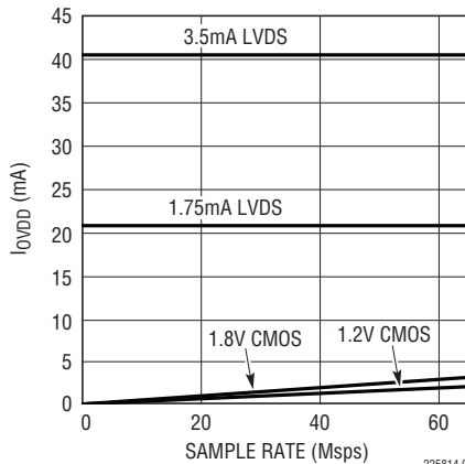
LTC2258-14: I_{OVPD} vs Sample Rate, 5MHz Sine Wave Input, -1dB, 5pF on Each Data Output
