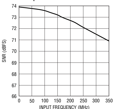
LTC2258-14: SNR vs Input Frequency, -1\text{dB} , 2\text{V} Range, 65\text{Mpsps}
