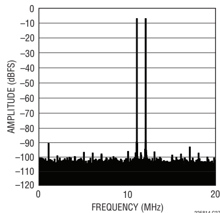
LTC2257-14: 8k Point 2-Tone FFT, f_{IN} = 68\text{MHz} , 69\text{MHz} , -1\text{dBFS} , 40\text{Mps}
