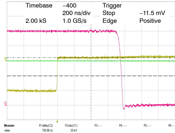
Figure 16. 10 mV Overdrive
