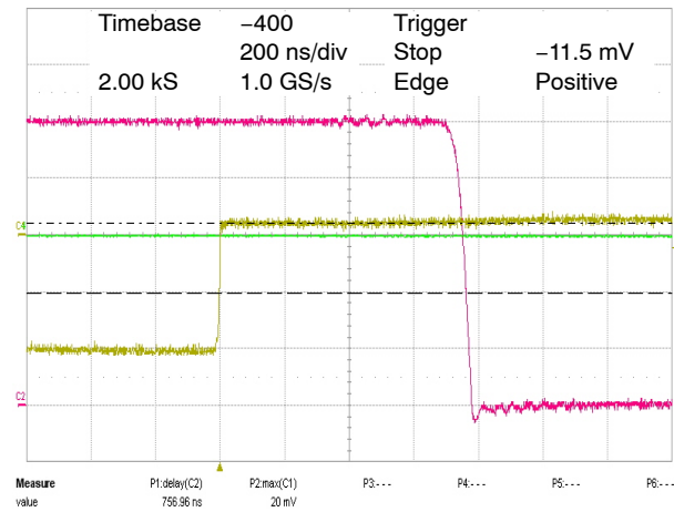
Figure 16. 10 mV Overdrive
