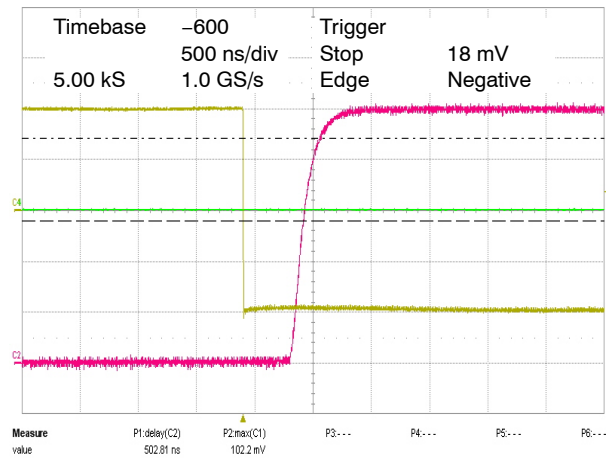
Figure 15. 100 mV Overdrive
