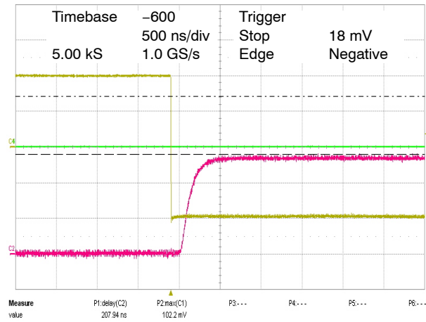
Figure 8. 20 mV Overdrive
