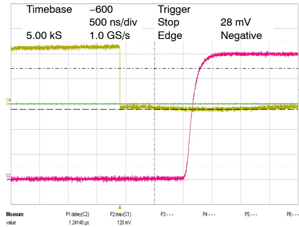
Figure 13. 10 mV Overdrive
