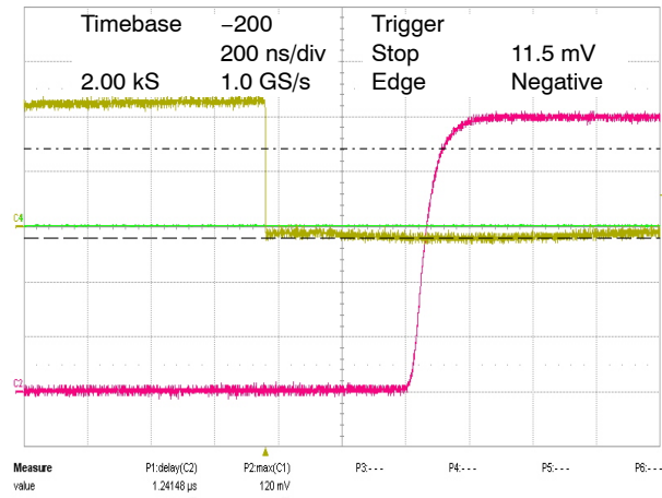
Figure 8. 20 mV Overdrive
