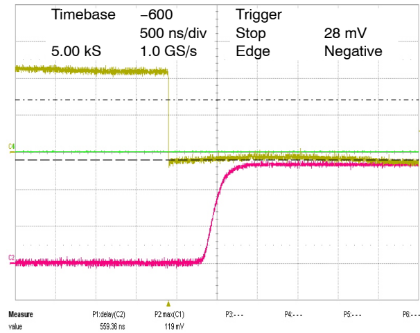
Figure 7. 10 mV Overdrive
