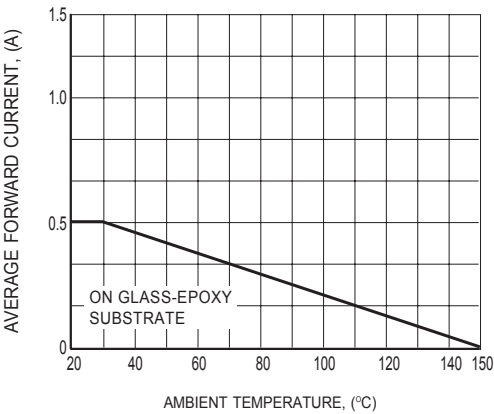
FIG.3 TYPICAL FORWARD CURRENT DERATING CURVE
