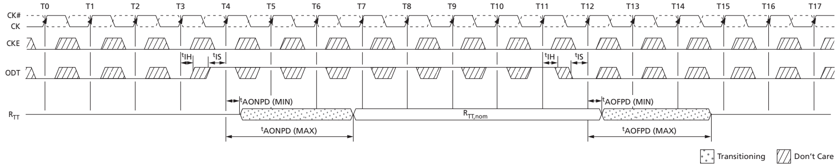
Figure 116: Asynchronous ODT Timing with Fast ODT Transition
