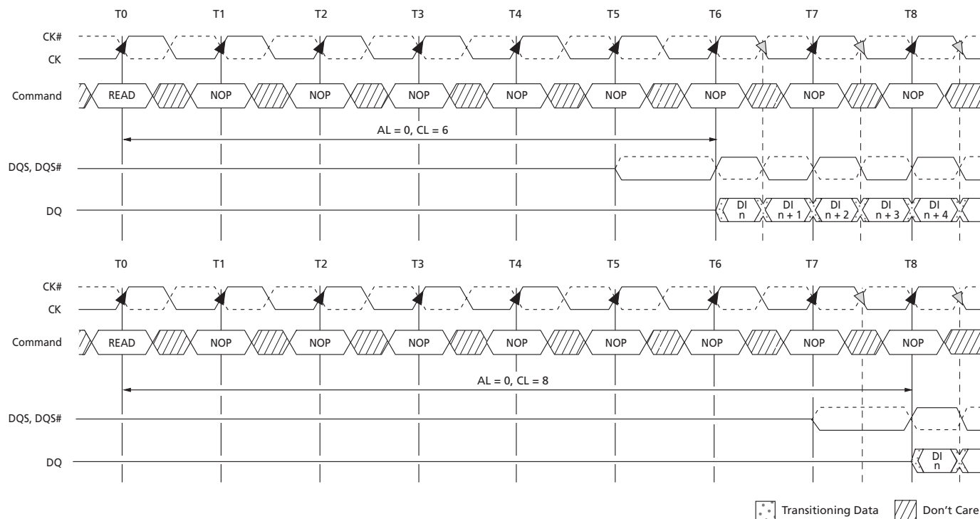
Figure 52: READ Latency
