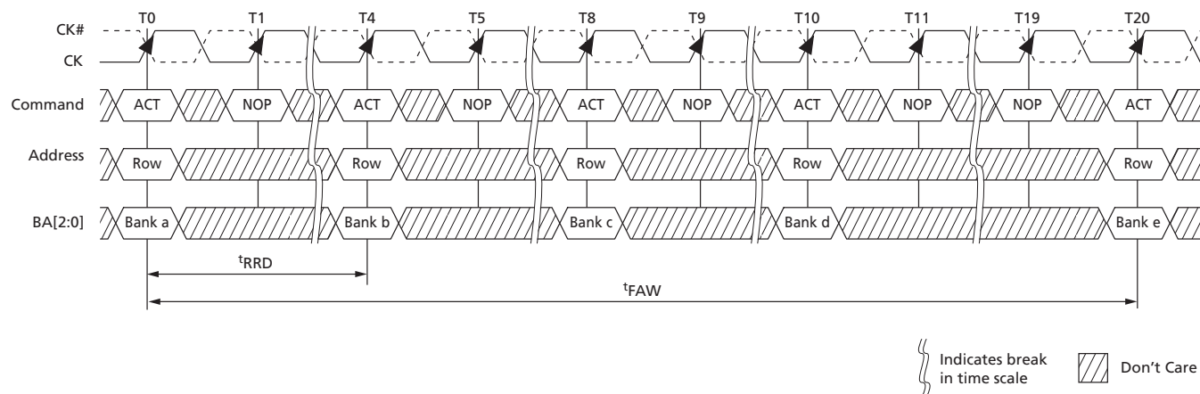
Figure 65: Example: t_{FAW}
