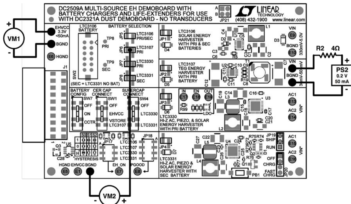
Figure 6. Setup for DC2509A Test Procedure with LTC3107
