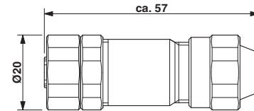
M12 x 1 socket, straight, shielded
