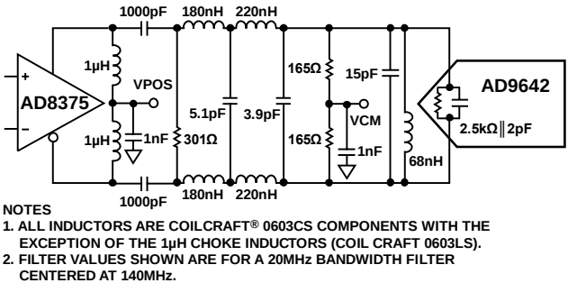
Figure 49. Differential Input Configuration Using the AD8375
