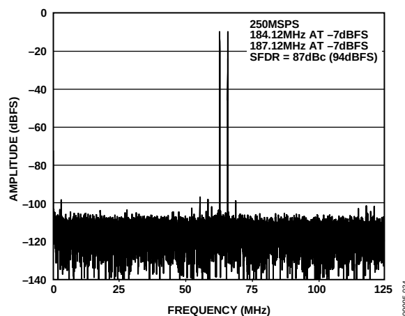
Figure 37. AD9642-250 Two Tone FFT with f_{IN1} = 184.12 MHz, f_{IN2} = 187.12 MHz
