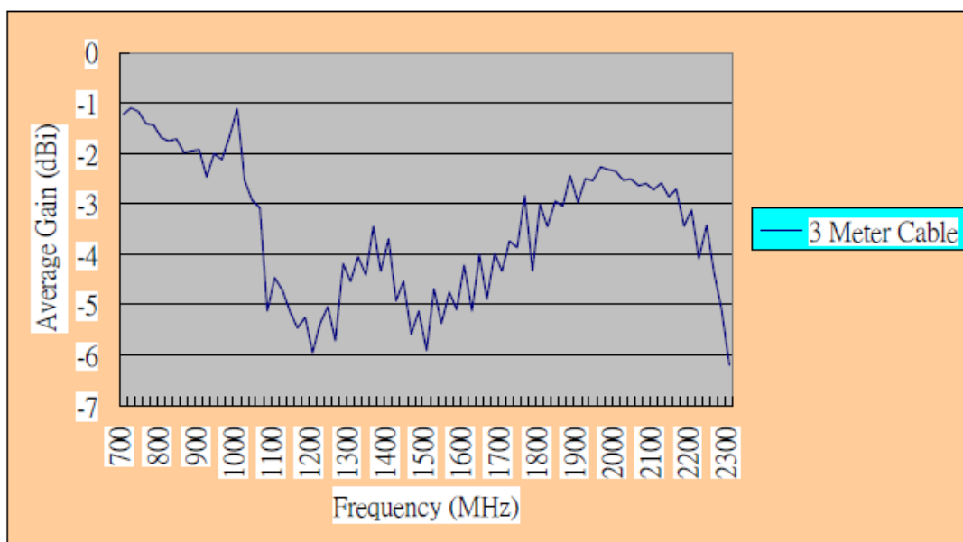
GSM/ UMTS Average Gain (with length 3 meter CFD-200 Cable)
