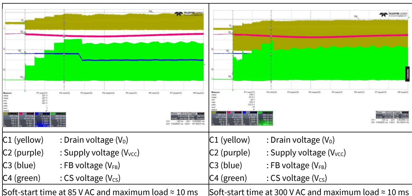
Figure 19 Soft-start
