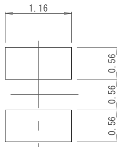
PCB Pattern
