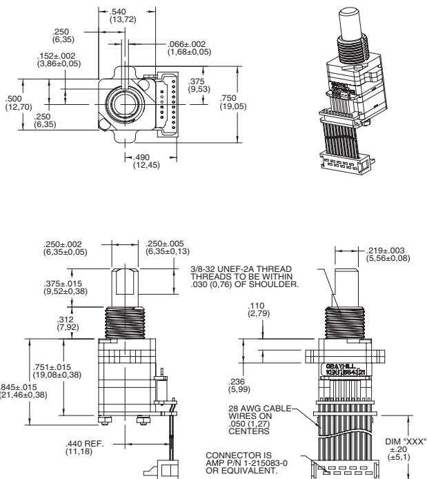
SERIES 62HR WITH .050 CENTER RIBBON CABLE
