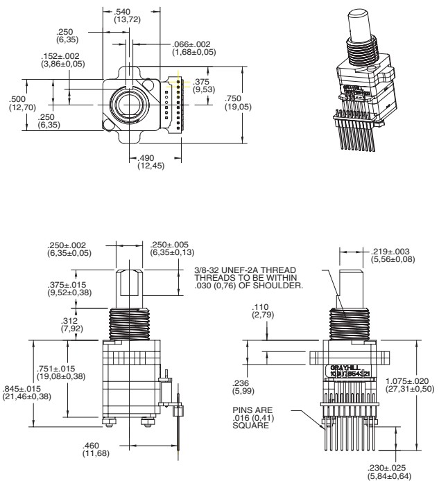
SERIES 62HR WITH .050 CENTER TERMINAL PINS
