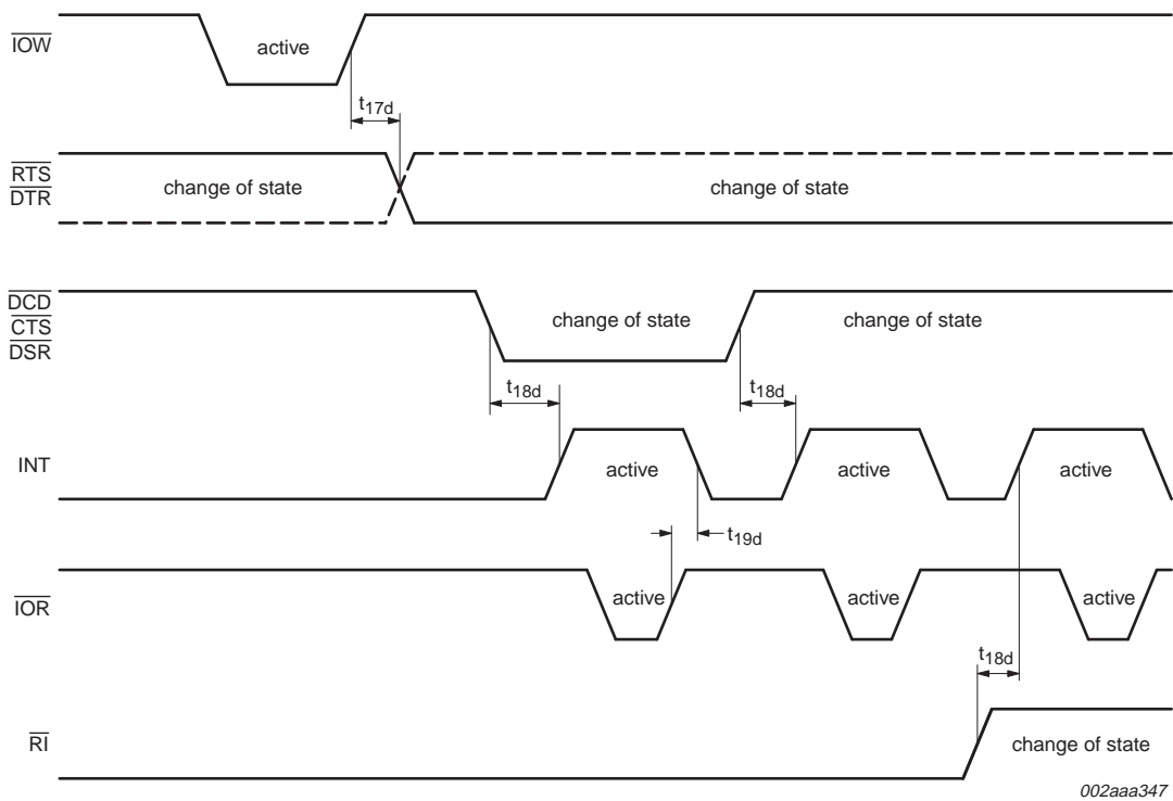
Fig 12. Modem input/output timing
