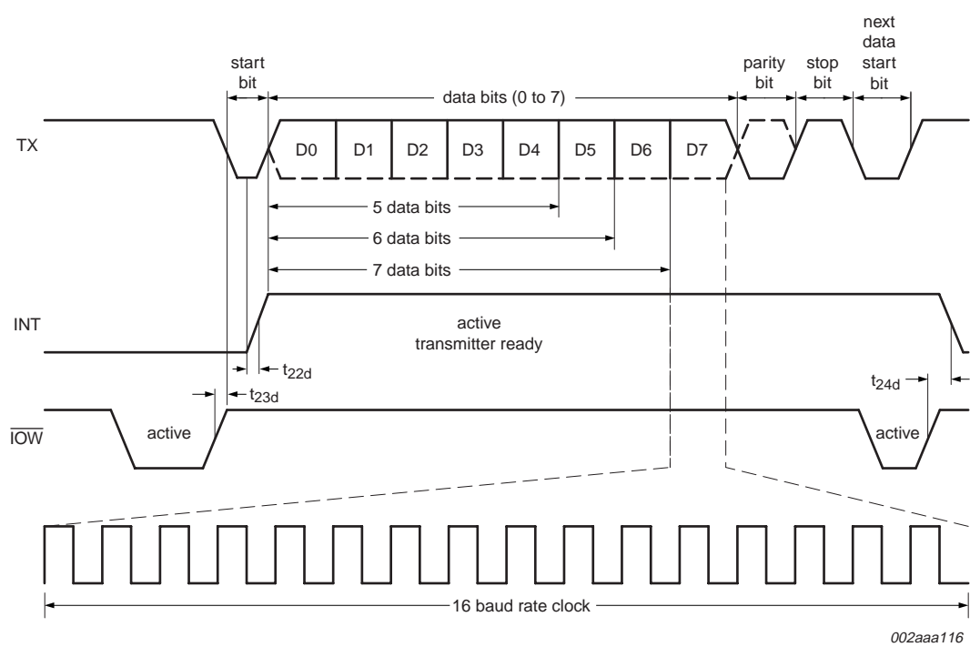
Fig 17. Transmit timing
