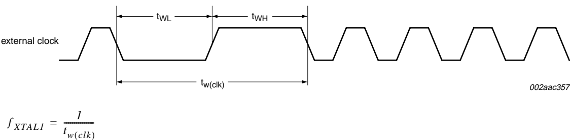
Fig 13. External clock timing
