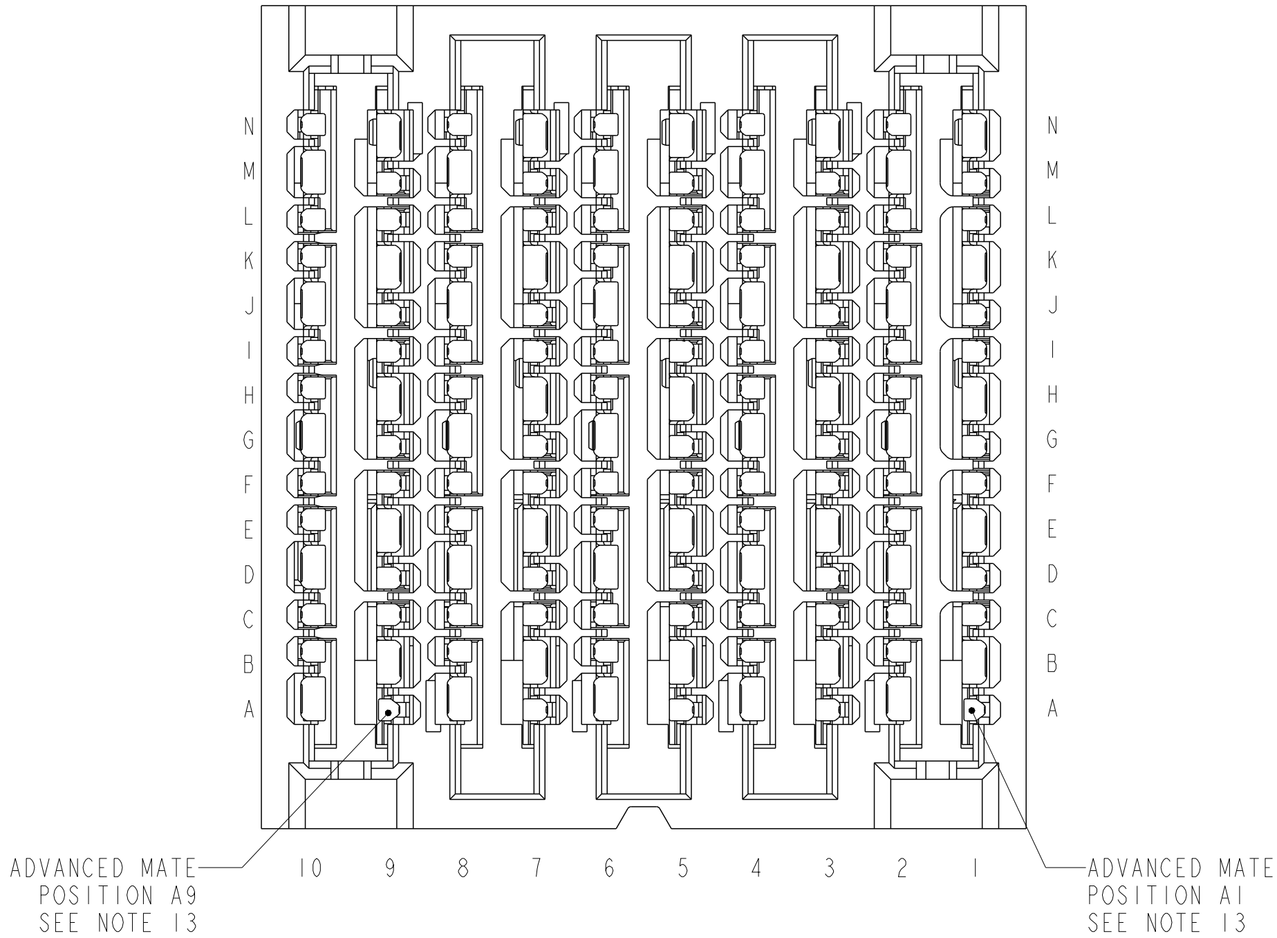
10135218-201LF ADVANCED MATE RECEPTACLE ADVANCED MATE POSITIONS ARE POSITIONS A1 AND A9 ONLY FOR ALL DIMENSIONS SEE 10135218-101LF ON SHEET 1
