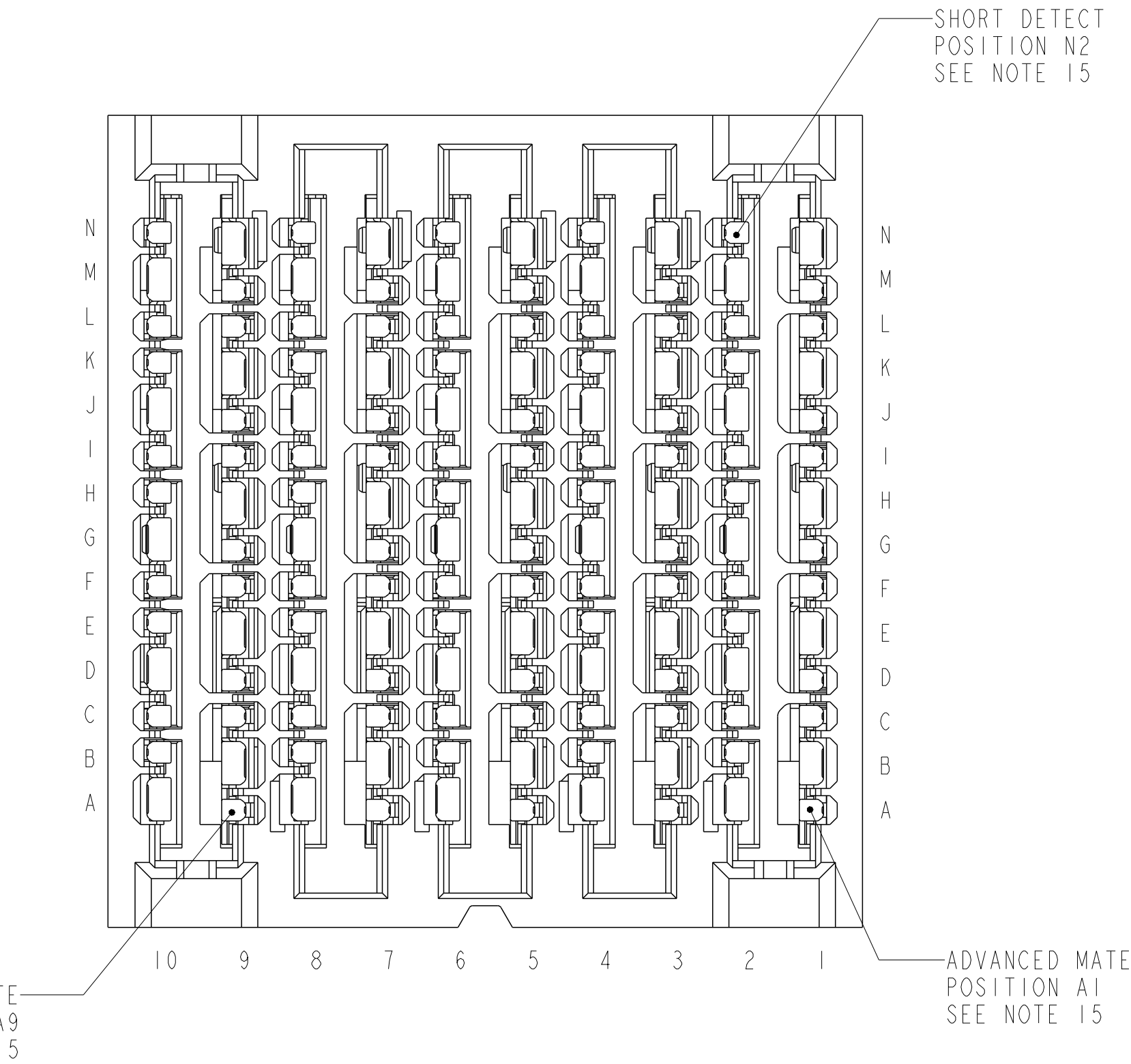
10135218-401LF ADVANCED MATE/SHORT DETECT RECEPTACLE ADVANCED MATE POSITIONS ARE POSITIONS A1 AND A9 ONLY SHORT DETECT POSITION IS N2 FOR ALL DIMENSIONS SEE 10135218-101LF ON SHEET 1
