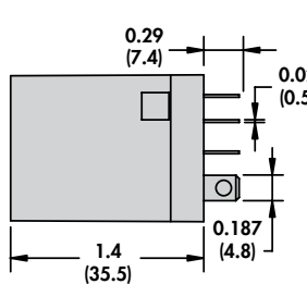
Plain Cover Dimensions
