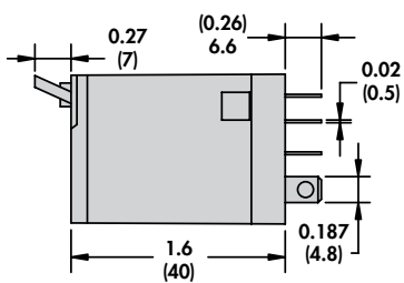
Full Featured Dimensions
