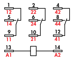
Wiring Diagram Bottom View
