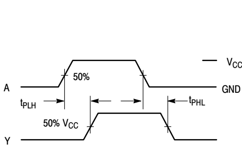
Figure 4. Switching Waveforms
