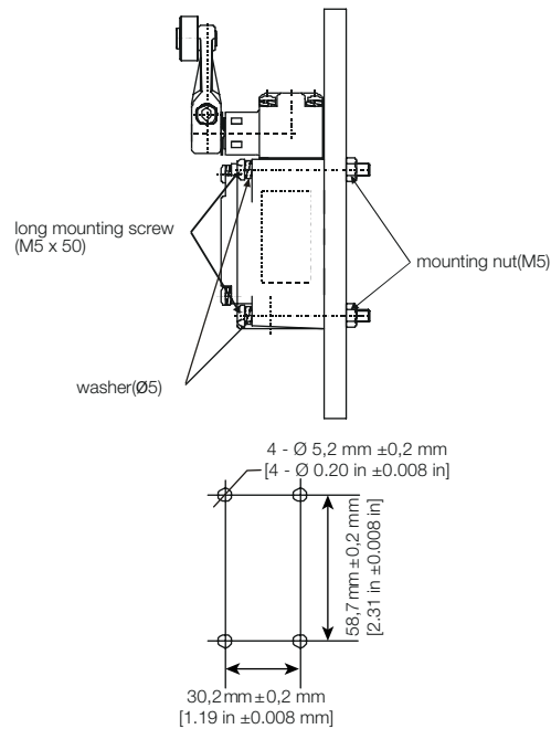
Figure 17. Through-Hole Mount
