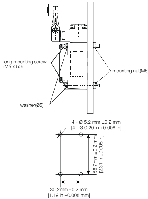
Figure 17. Through-Hole Mount
