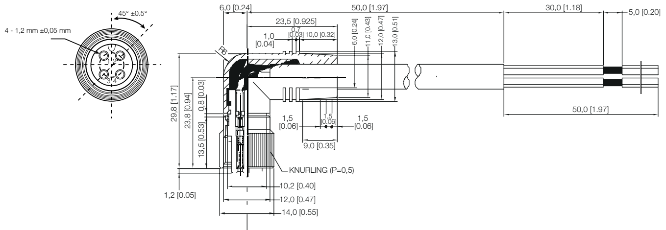
Figure 22. ZLC-4DLF-__
