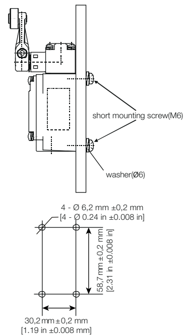
Figure 18. Rear Mount
