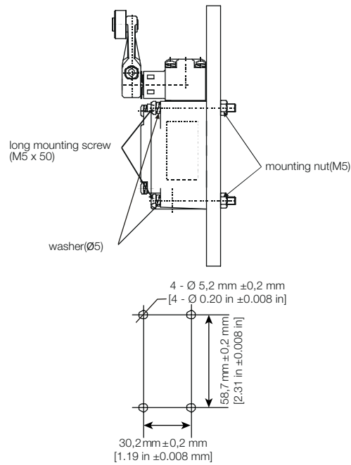
Figure 17. Through-Hole Mount
