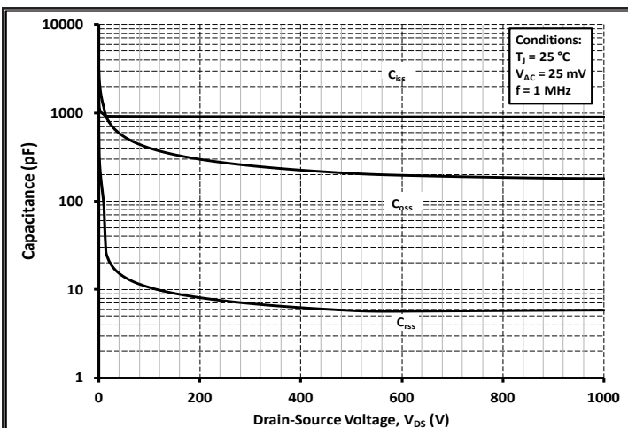
Figure 17. Capacitances vs. Drain-Source Voltage (0 - 1 kV)
