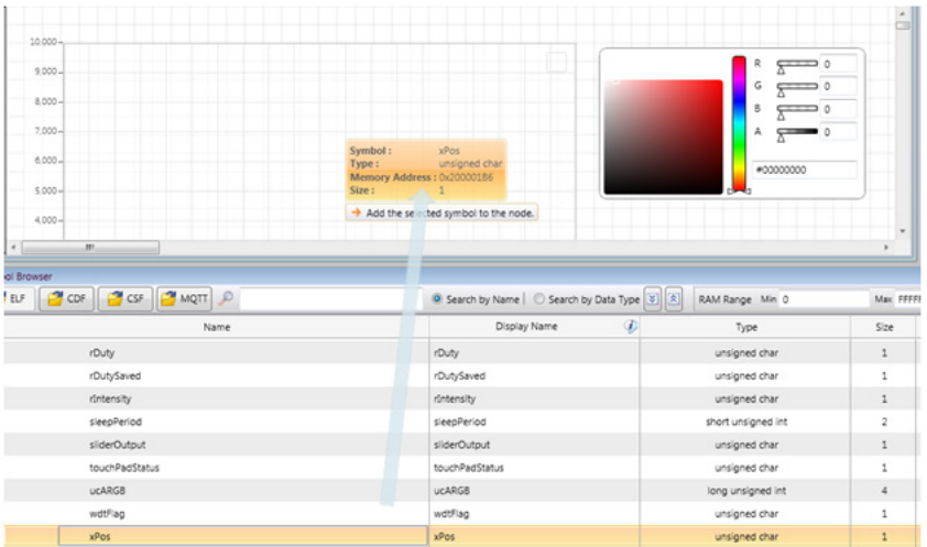
Figure 6-69. Assigning x Position output to Line Chart control
