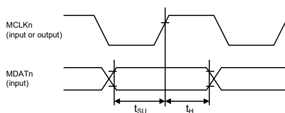
Figure 2.80 Reception Timing (MCLKn Rising Synchronous)
