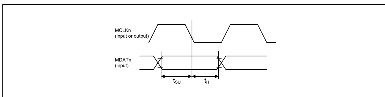
Figure 2.81 Reception Timing (MCLKn Falling Synchronous)
