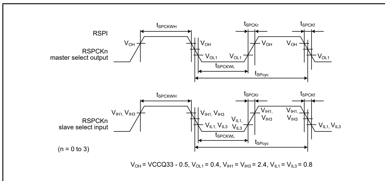
Figure 2.52 RSPIa Clock Timing
