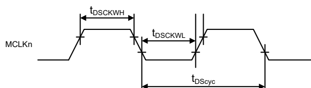
Figure 2.79 Clock Input/Output Timing
