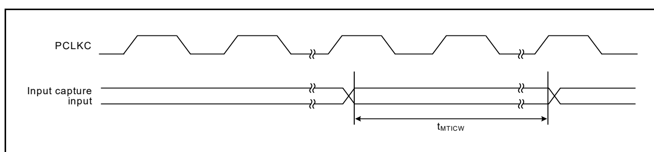
Figure 2.43 MTU3a Input Capture Input Timing
