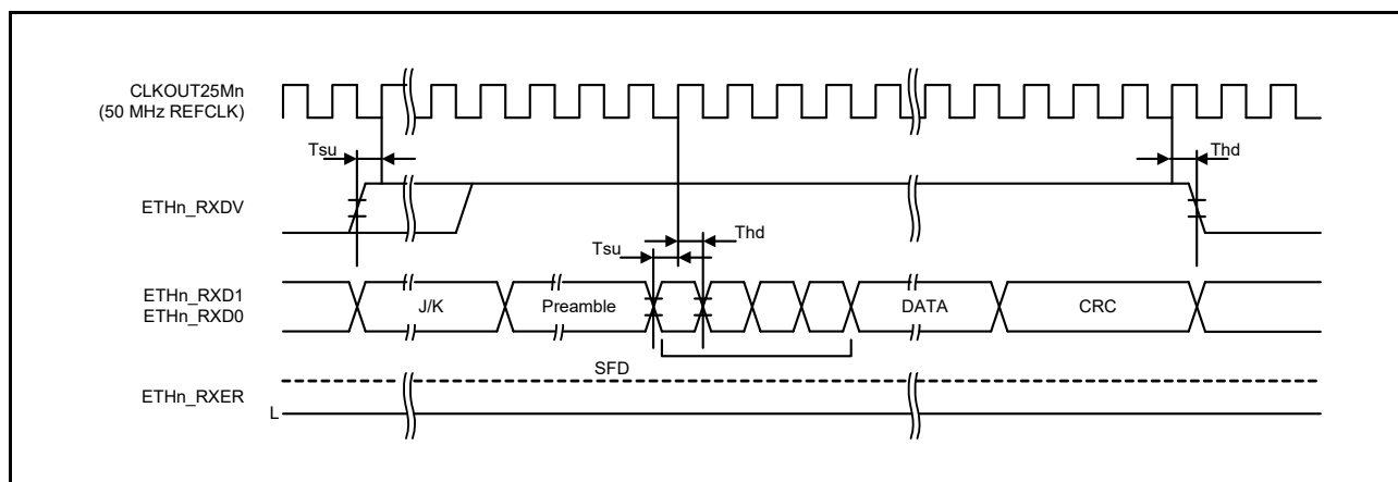
Figure 2.72 RMII Reception Timing (Normal Operation)
