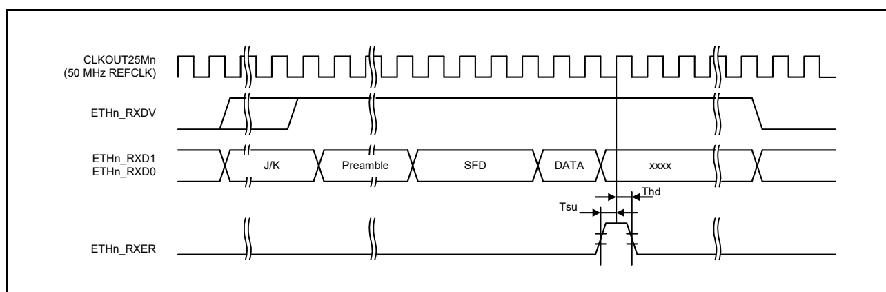
Figure 2.73 RMII Reception Timing (Error Occurrence)
