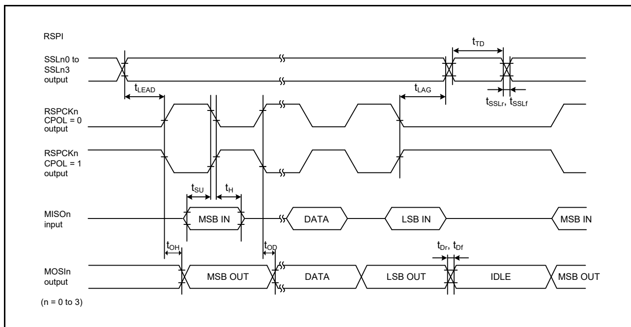
Figure 2.53 RSPIa Timing (Master, CPHA = 0)
