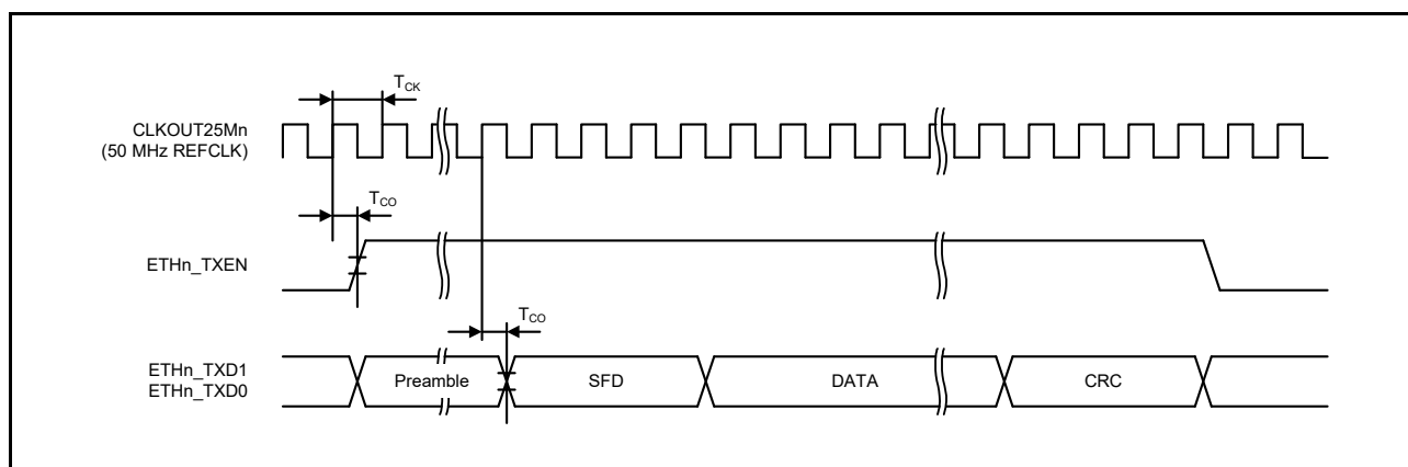
Figure 2.71 RMII Transmission Timing
