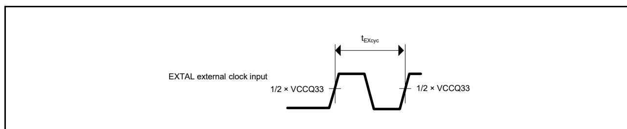
Figure 2.5 EXTAL External Clock Input Timing
