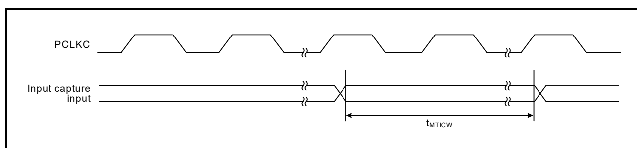
Figure 2.43 MTU3a Input Capture Input Timing
