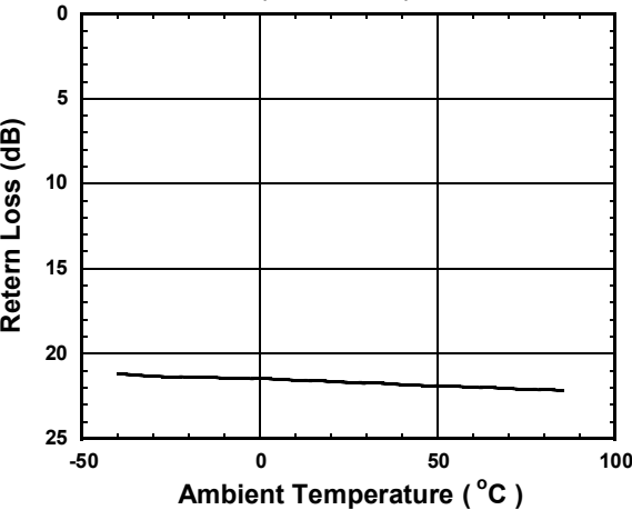
BT Port Return Loss vs. Ambient Temperature
