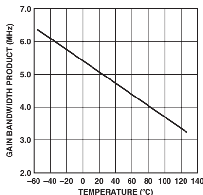
TPC 9. Gain Bandwidth Product vs. Temperature
