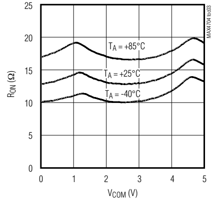
ON-RESISTANCE vs. V_{COM} ( V_+ = 5V )
