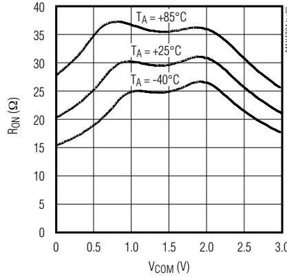
ON-RESISTANCE vs. V_{COM} ( V_+ = 3V )
