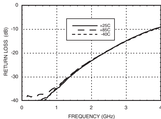
Return Loss
