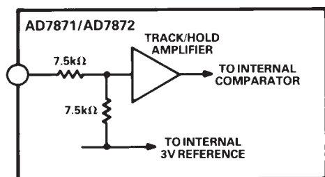
Figure 4. Analog Input
