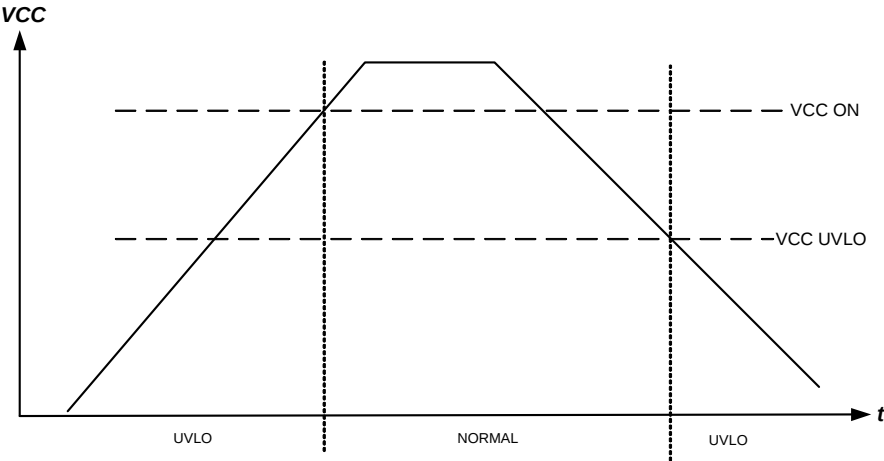
Figure 3: Vcc UVLO
