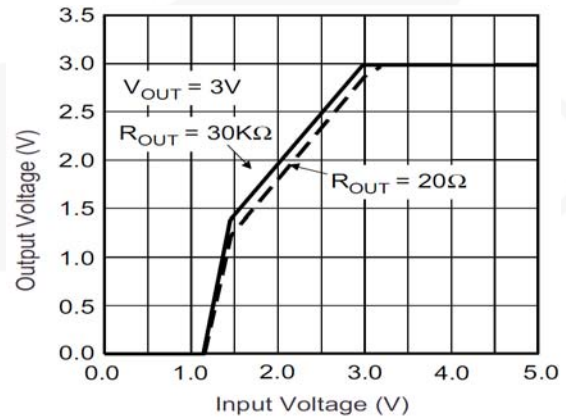
Figure 20. Dropout Characteristics
