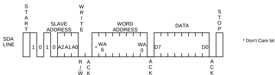
Figure 36. Byte write cycle
