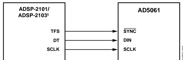
Figure 40. AD5061-to-ADSP-2101/ADSP-2103 Interface
