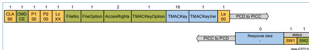
Figure 27. CreateTransactionMACFile command protocol
