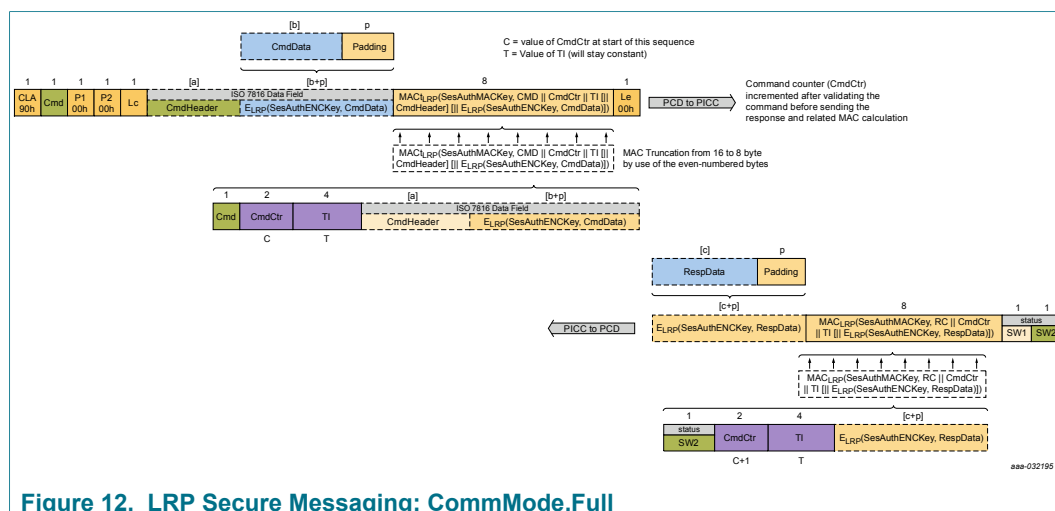
Figure 12. LRP Secure Messaging: CommMode.Full
