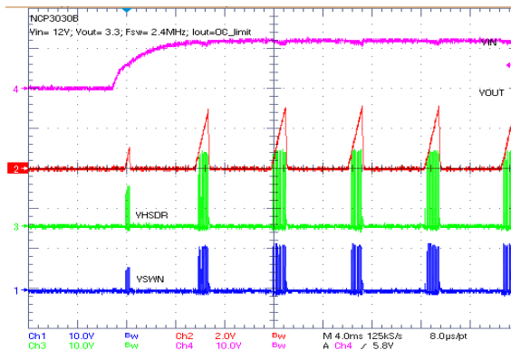
Figure 17. Startup Waveforms (NCP3030B)
