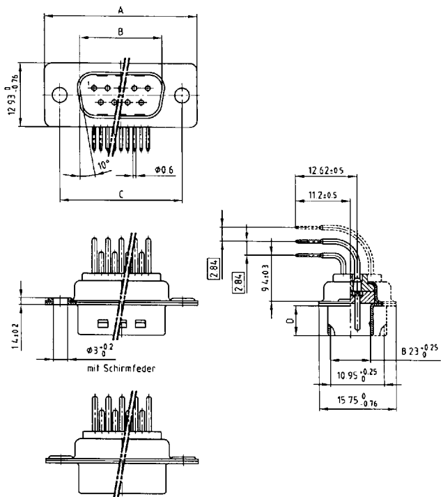
Plug connector
