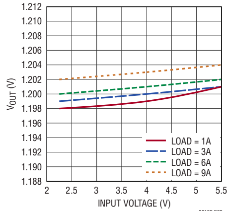
V_{OUT} Line Regulation, V_{OUT} = 1.2\text{V}
