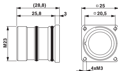
Dimensional drawing
