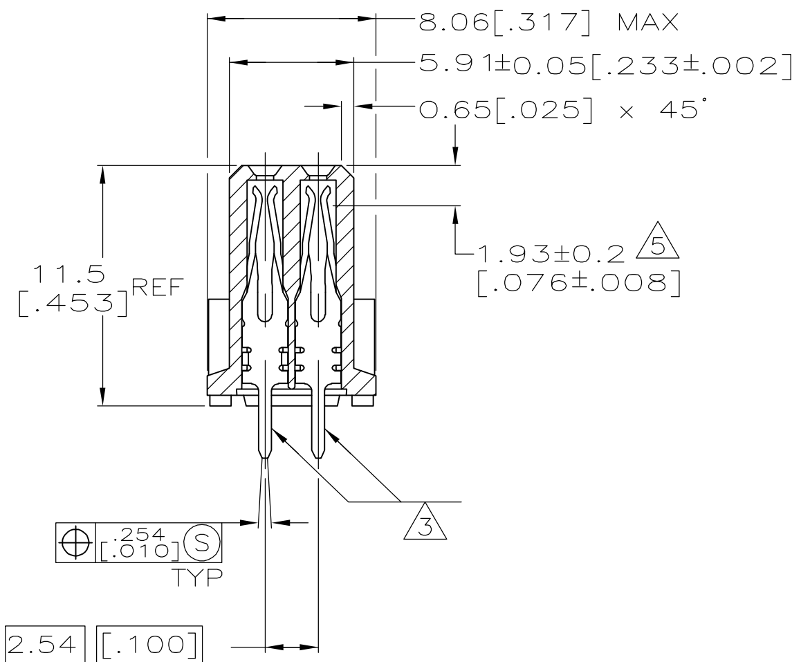
SECTION X-X
