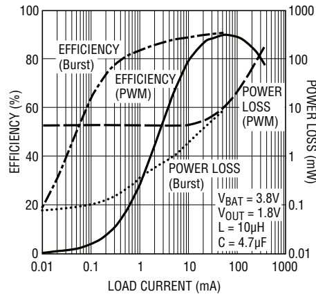
Buck Efficiency vs Load Current ( V_{\text{OUT}} = 1.8\text{V} )
