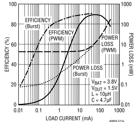
Buck Efficiency vs Load Current ( V_{\text{OUT}} = 1.5\text{V} )
