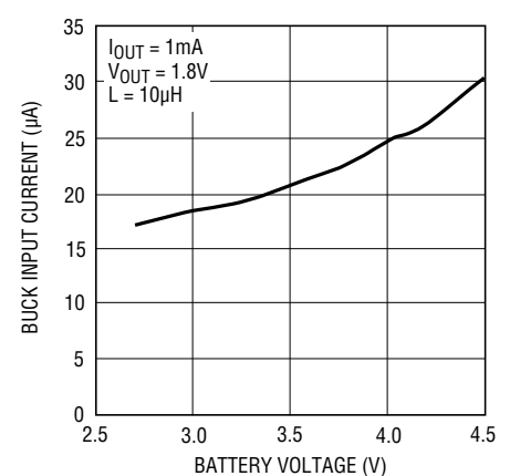
No-Load Buck Input Current (Burst Mode Operation) vs Battery Voltage
