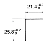
Panel Cutout
